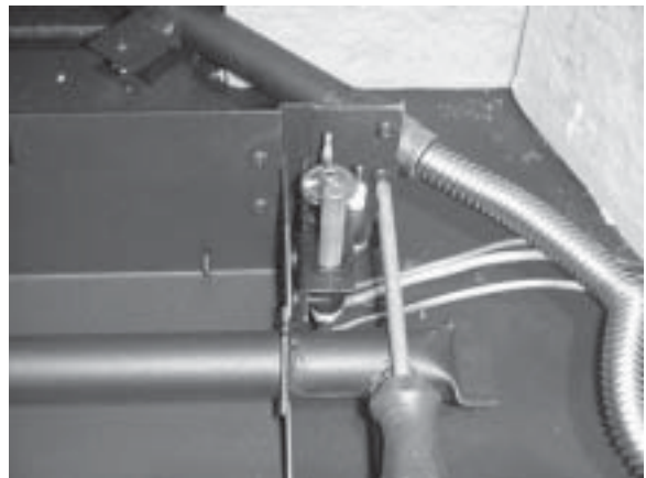
ATTACH PILOT BRACKET TO BURNER ASSEMBLY
