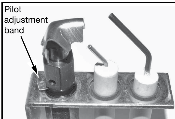
Figure 22: Pilot band in natural gas position.
