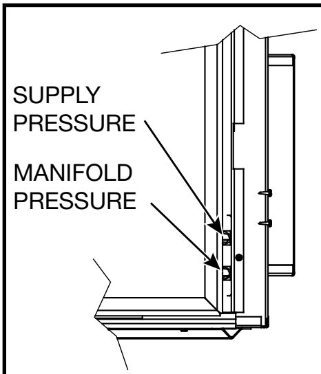
Figure 40: Gas test ports.
