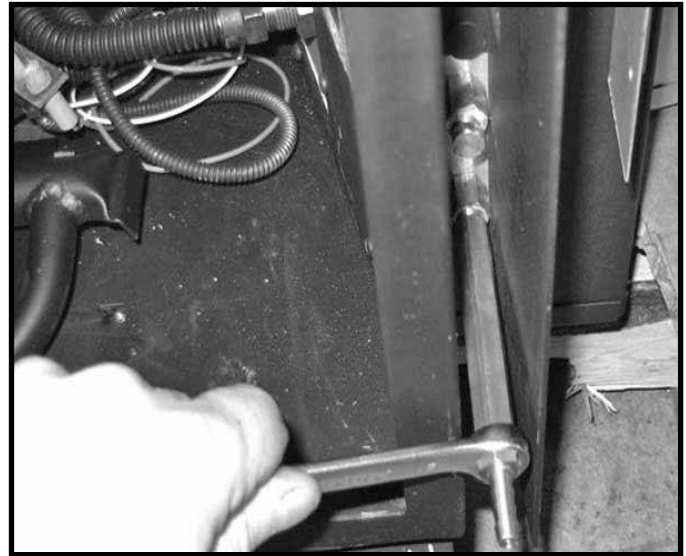
Figure 39: Adjusting manifold pressure.
