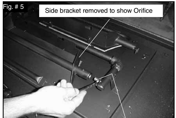
Burner Orifice
