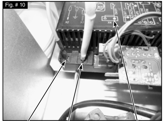
IGNITION WIRE (RED) FLAME SENSOR WIRE (WHITE) INTERFACE MODULE
