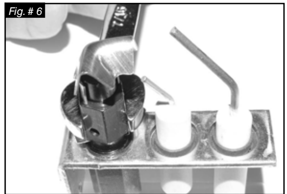
Burner Orifice
