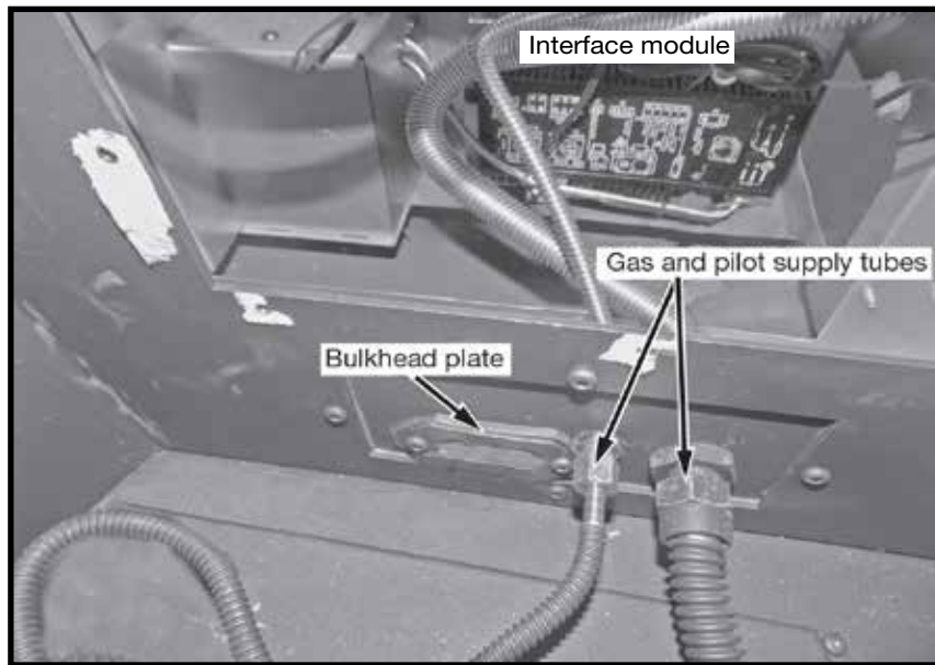
Figure 6: Attach gas supply tubes to bulkhead
