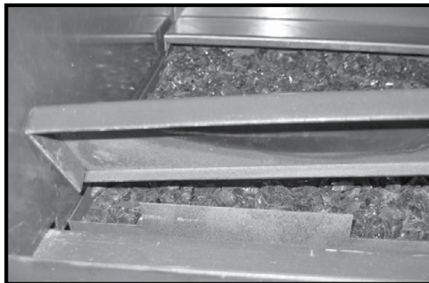
Figure 10: Positioning front trim.
