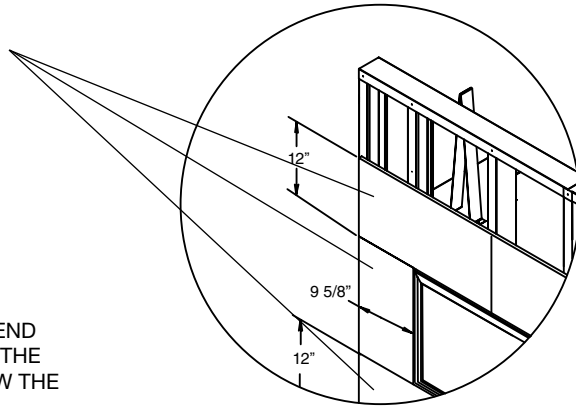
Figure 12: TCWS54OD Non-combustible board dimensions.
