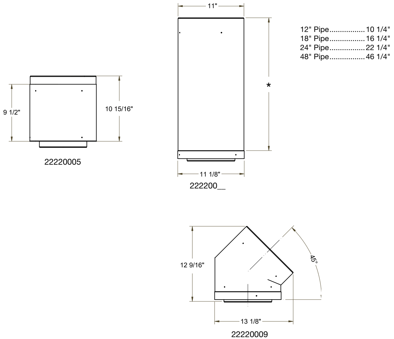
Figure 45: Pipe dimensions.
