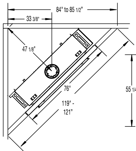
Figure 15: TCWS54 OD w Screen framing dimensions.
