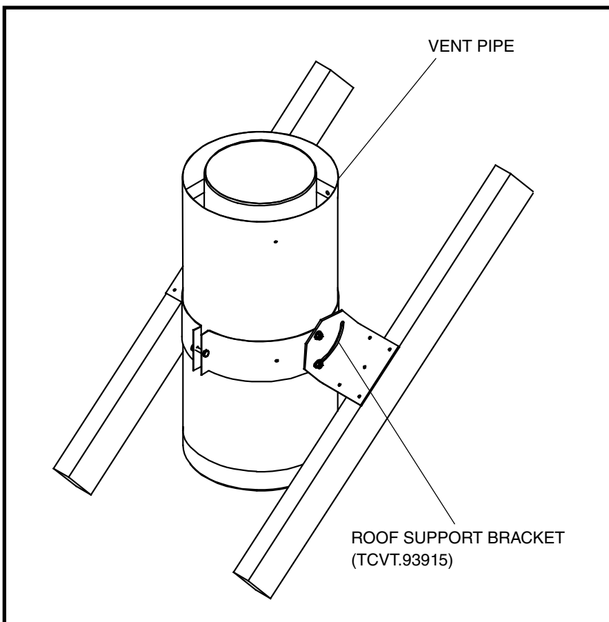
Figure 32: Roof support bracket.
