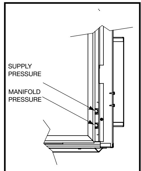
Figure 27: Test ports.
