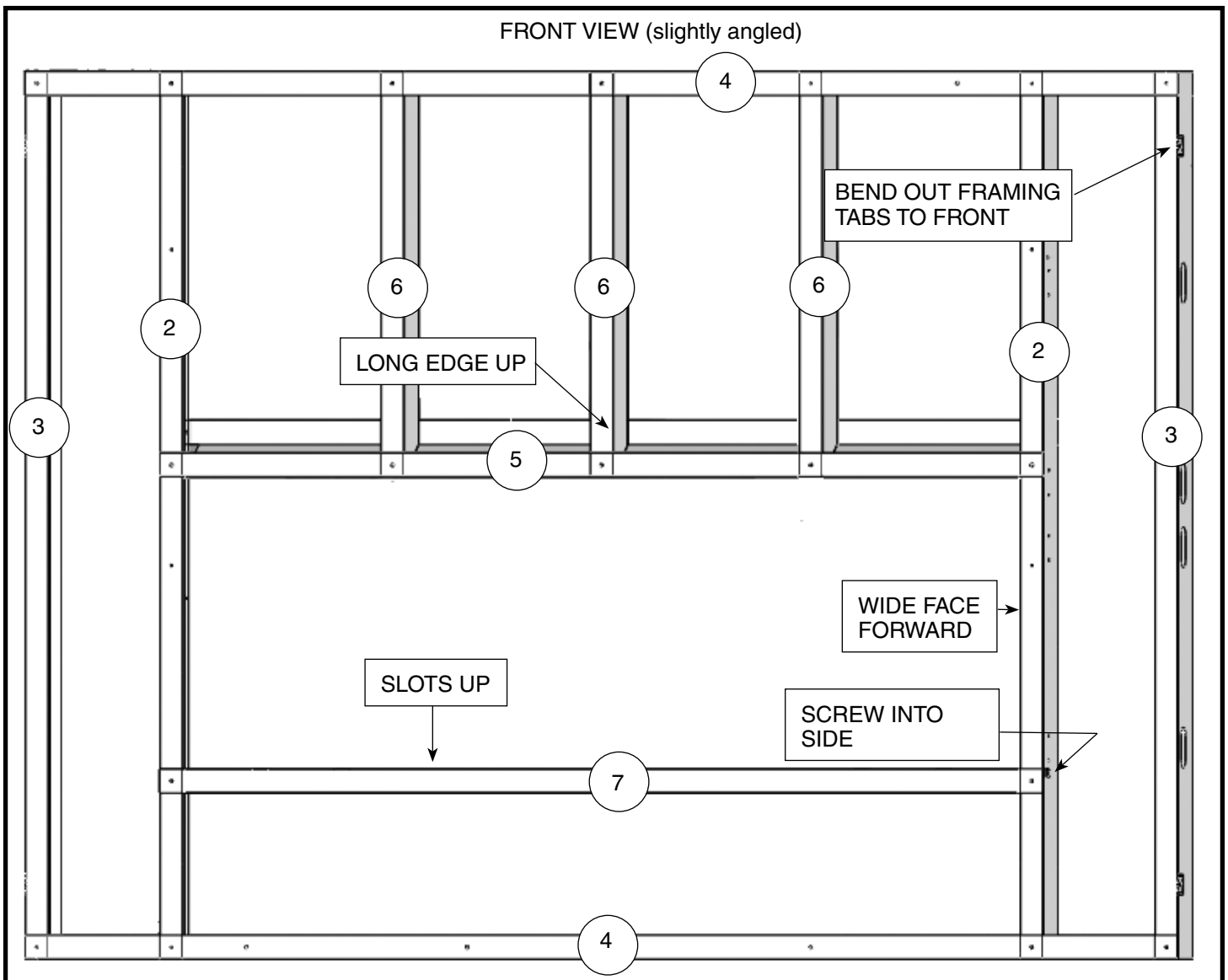
Figure 17: TCWS54OD Steel frame assembled.
