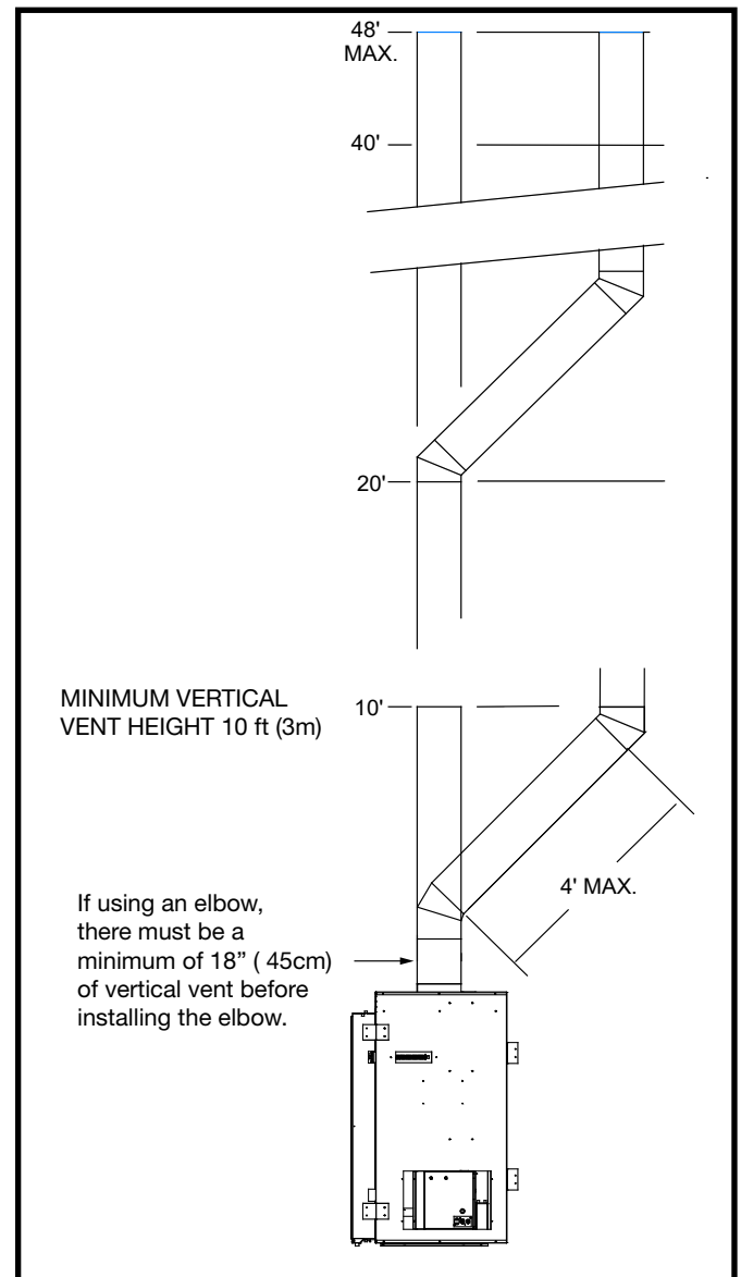
Figure 30: TCWS54OD Venting chart.
