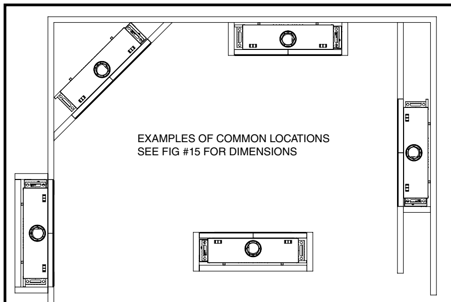
Figure 10: TCWS54OD Possible locations.
