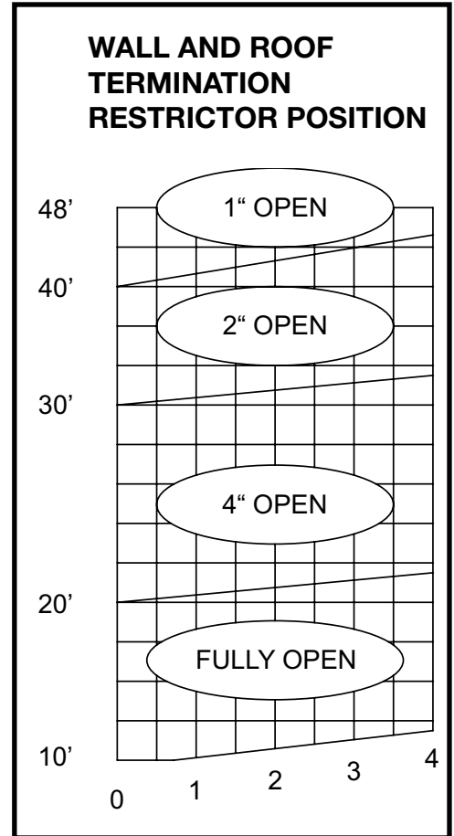
Figure 36: Restrictor position chart.
