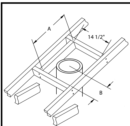
Figure 31: Roof opening frame.
