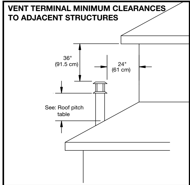
Figure 34: Roof terminal clearances.
