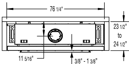
Figure 15: TCWS54 OD w Screen framing dimensions.
