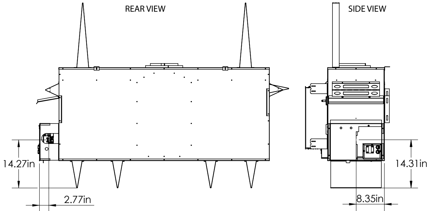
Figure 28: TCWS54 OD Main gas connection dimensions.
