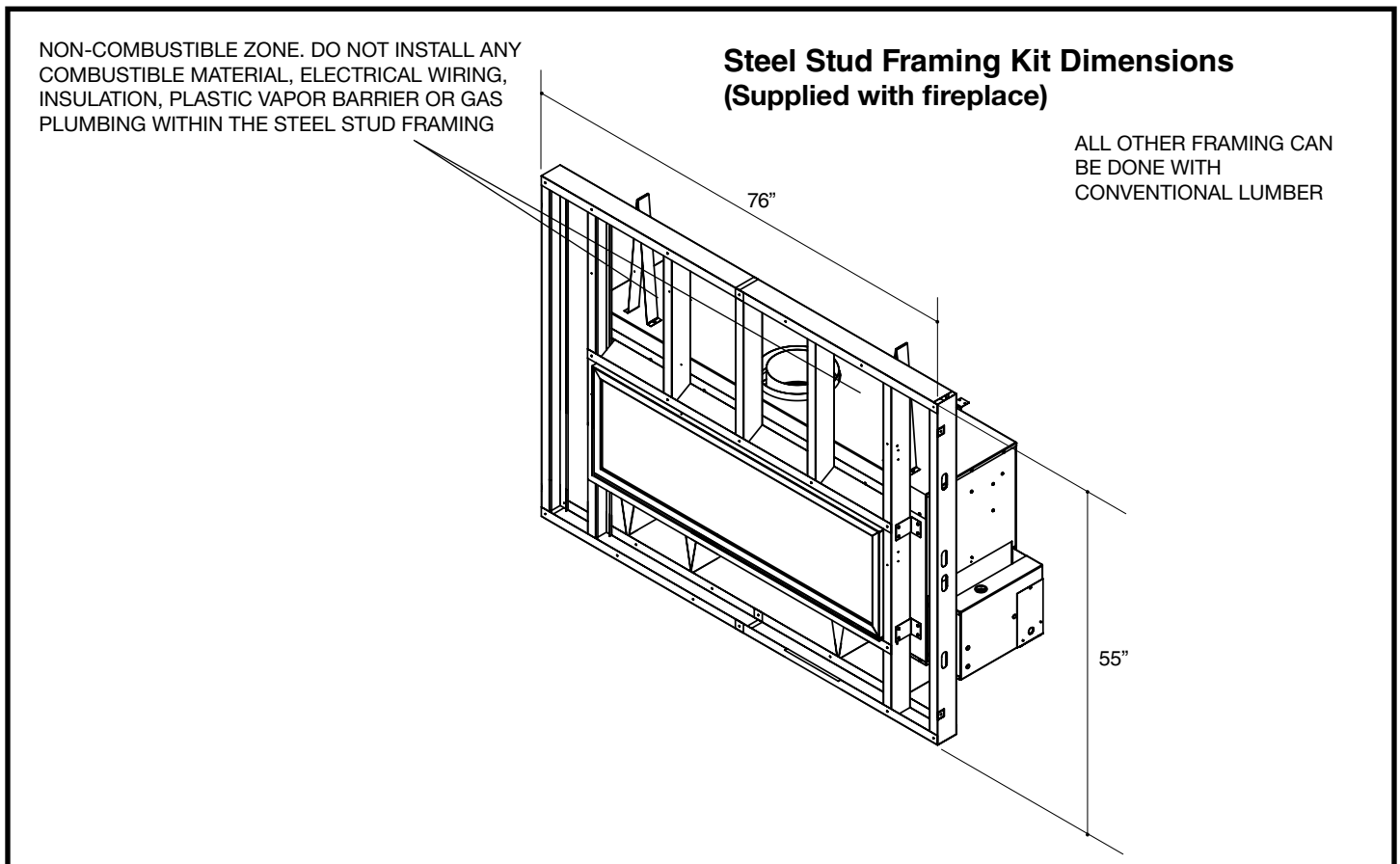
Figure 11: TCWS54OD with supplied steel frame.
