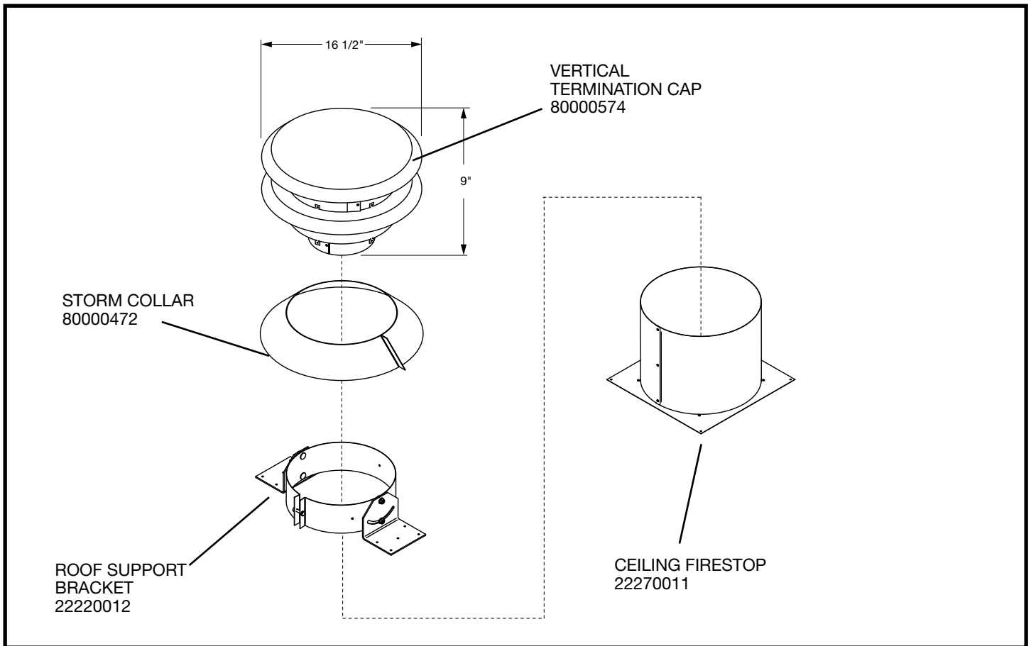
Figure 44: Vent terminal kit.
