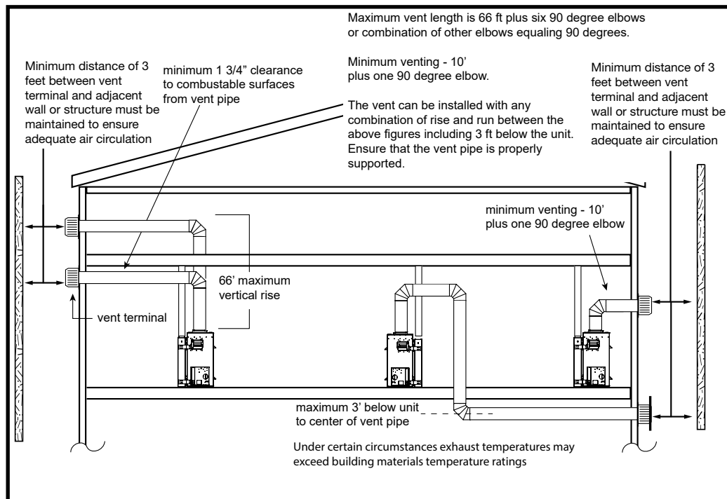
Figure 1: Venting configurations.
