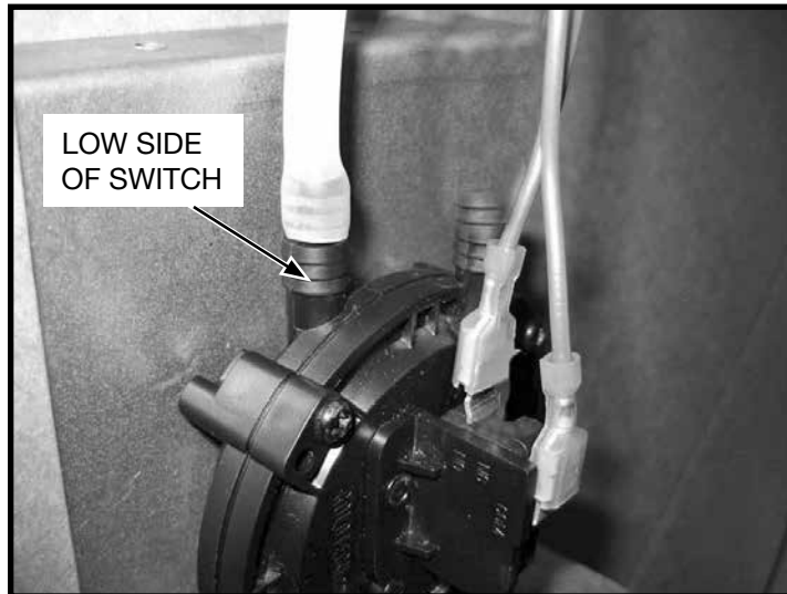
Figure 9: Switch sides.
